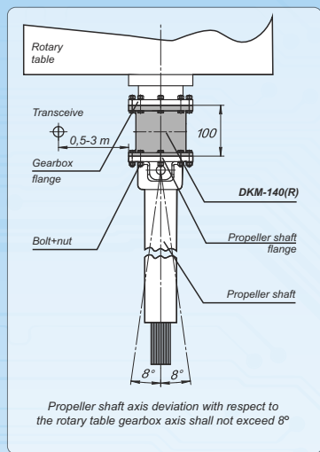
DKM-140(R) Torque sensor mounting on a rig.
